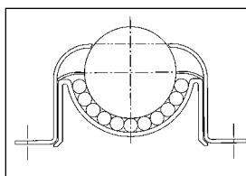
SINGLE BALL TRANSFER model BALL-1F
