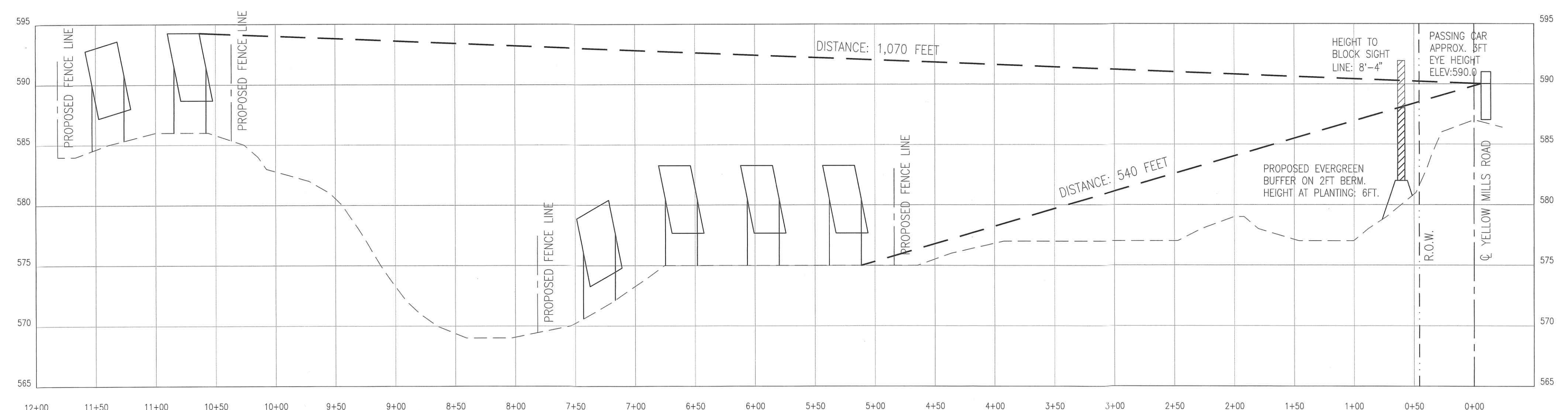
SIGHT LINE PROFILE FROM SOUTHEAST CORNER
