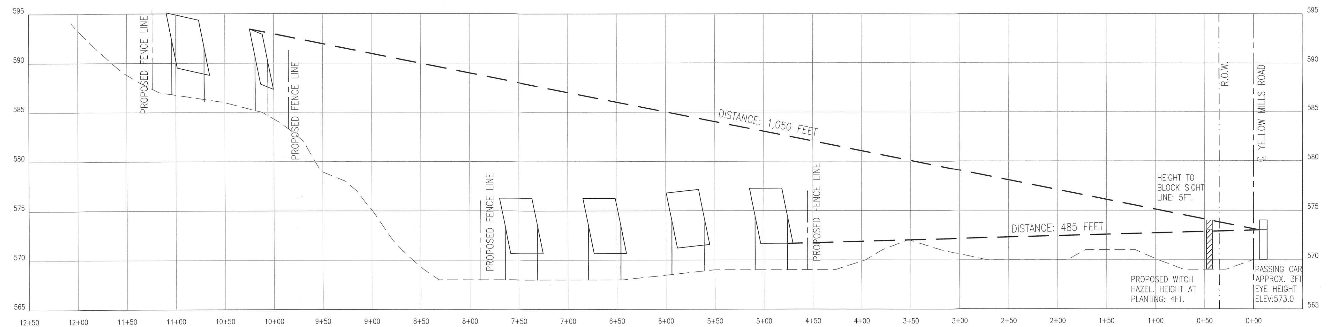
SIGHT LINE PROFILE FROM SOUTH of #466 YELLOW MILLS ROAD
