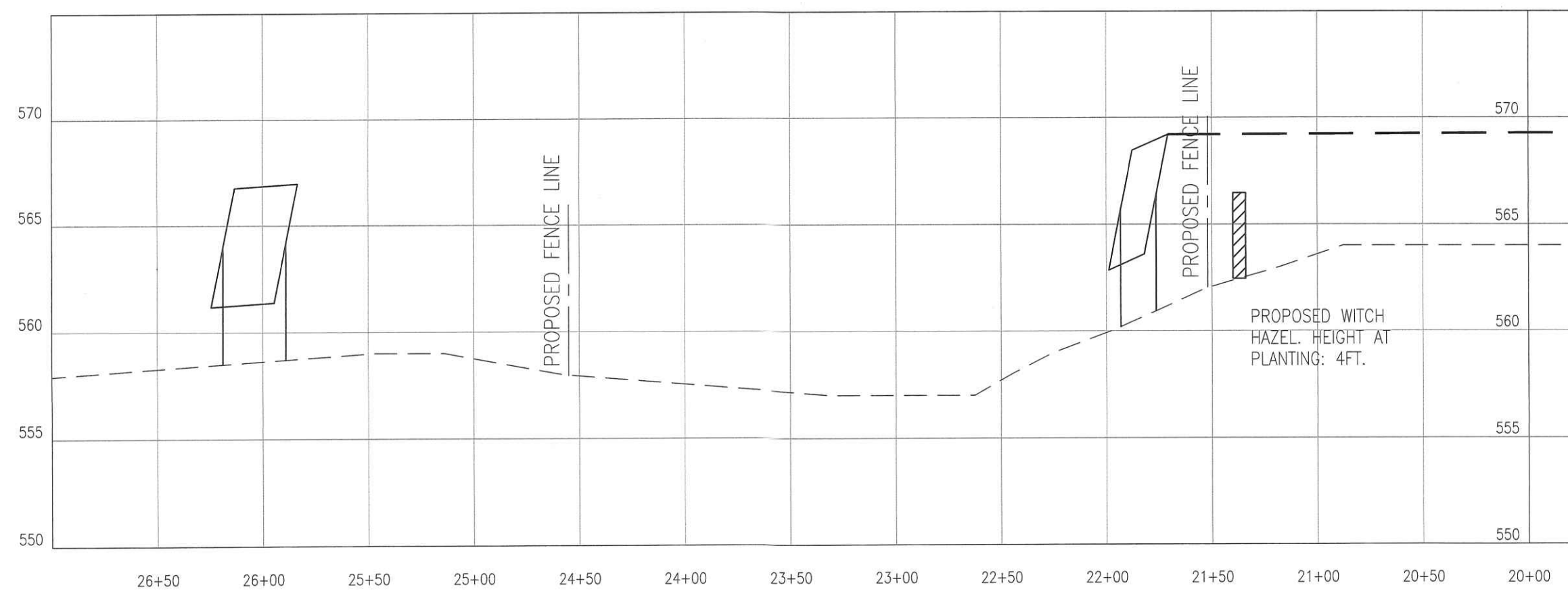
SIGHT LINE PROFILE for 4465 FOX ROAD
