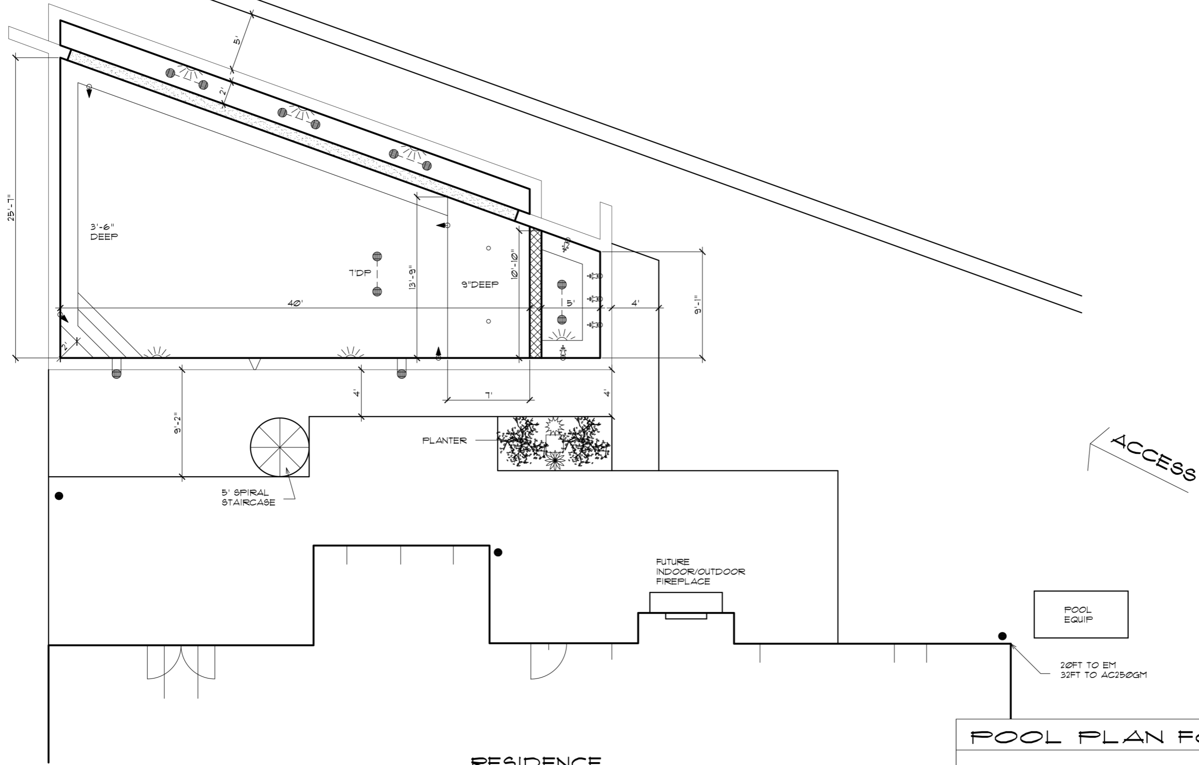
RESIDENCE POOL PLAN SCALE: 1/8" = 1'-0"
