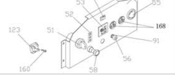
KGE3300Ti-13100 Control panel assembly
